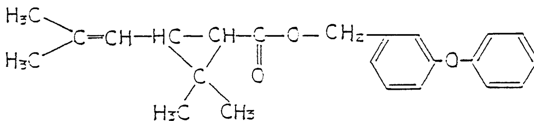
permethrin [3-phenoxybenzyl cis/trans-3-(2,2-dichlorovinyl)-2,2-dimethyl-1-cyclopropanecarboxylate];
