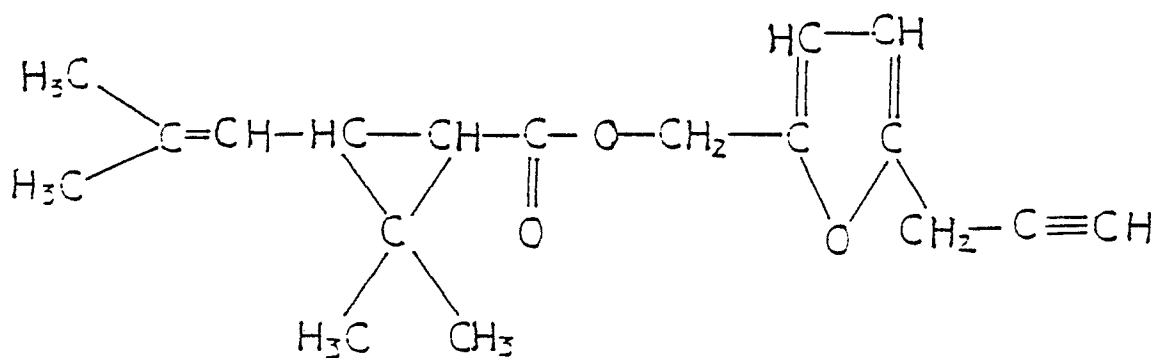
phenothrin [3-phenoxybenzyl d-cis/trans-chrysanthemate];
