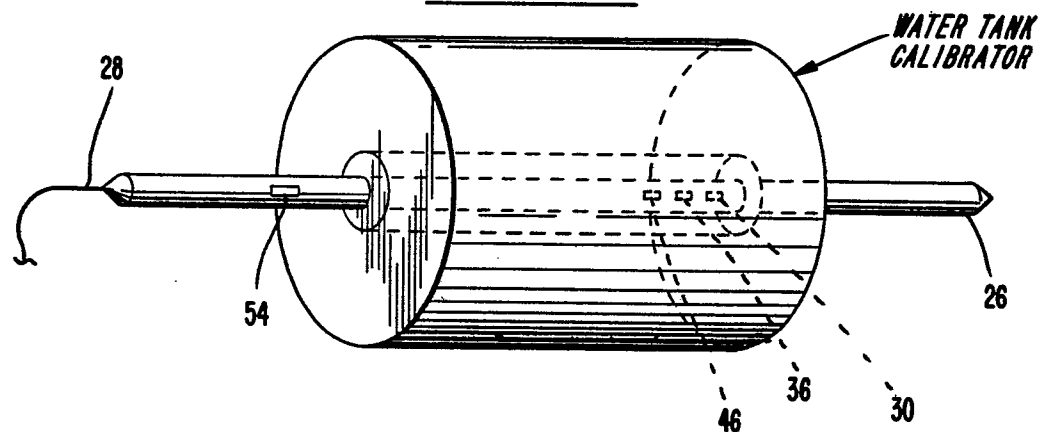
SHOP CALIBRATOR
