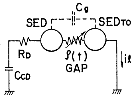
FIG. 10 (PRIOR ART)
