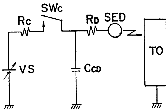
FIG. 9 (PRIOR ART)
