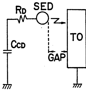
FIG. 1 (PRIOR ART)
