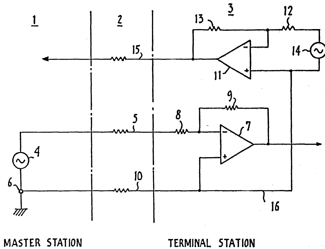
FIG. 1 PRIOR ART
