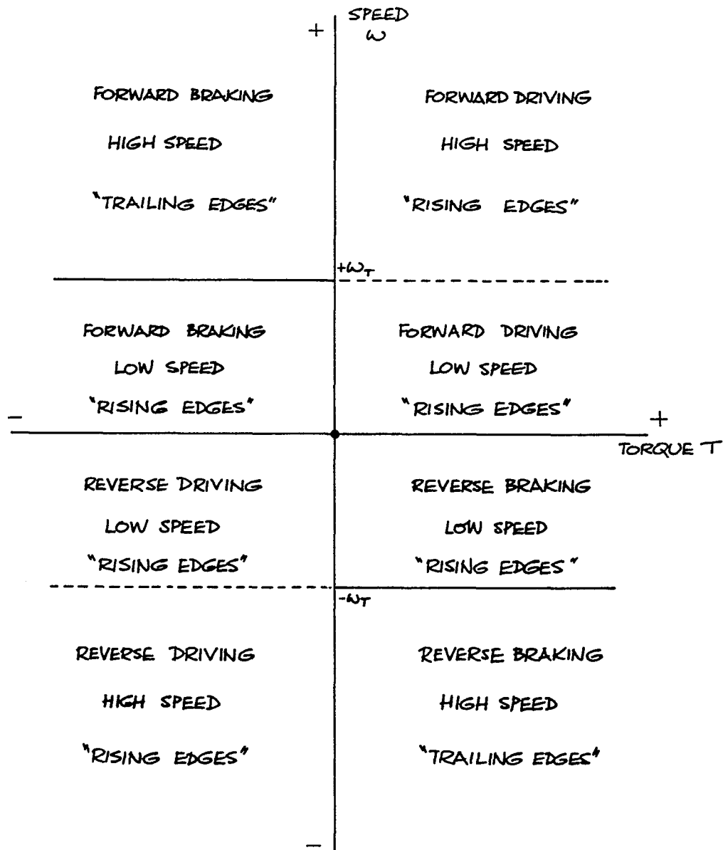
CURRENT SELECTION REGIONS IN FOUR QUADRANT OPERATION
