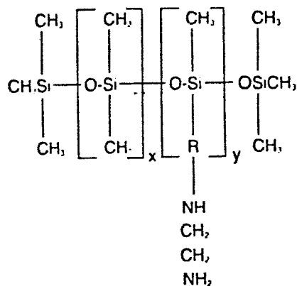
Trimethylsilylamodimethicone
