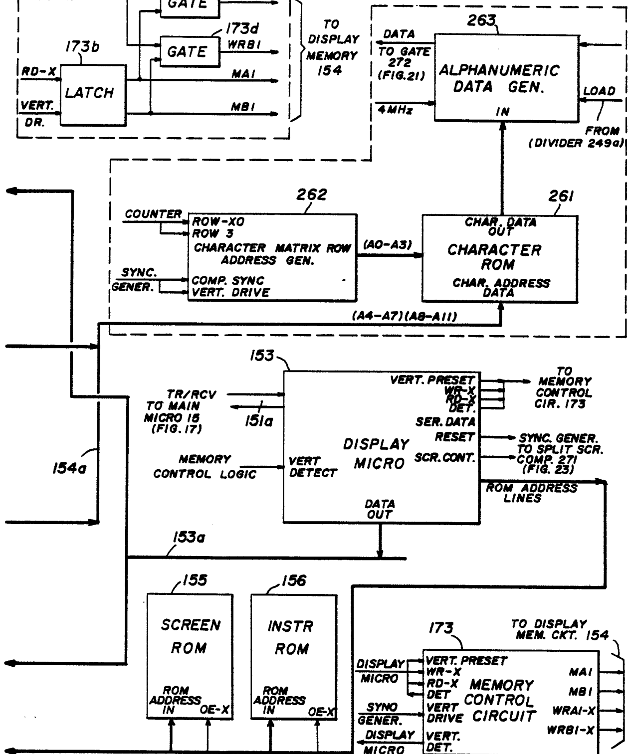
FIG. 24 CHARACTER GENERATOR
