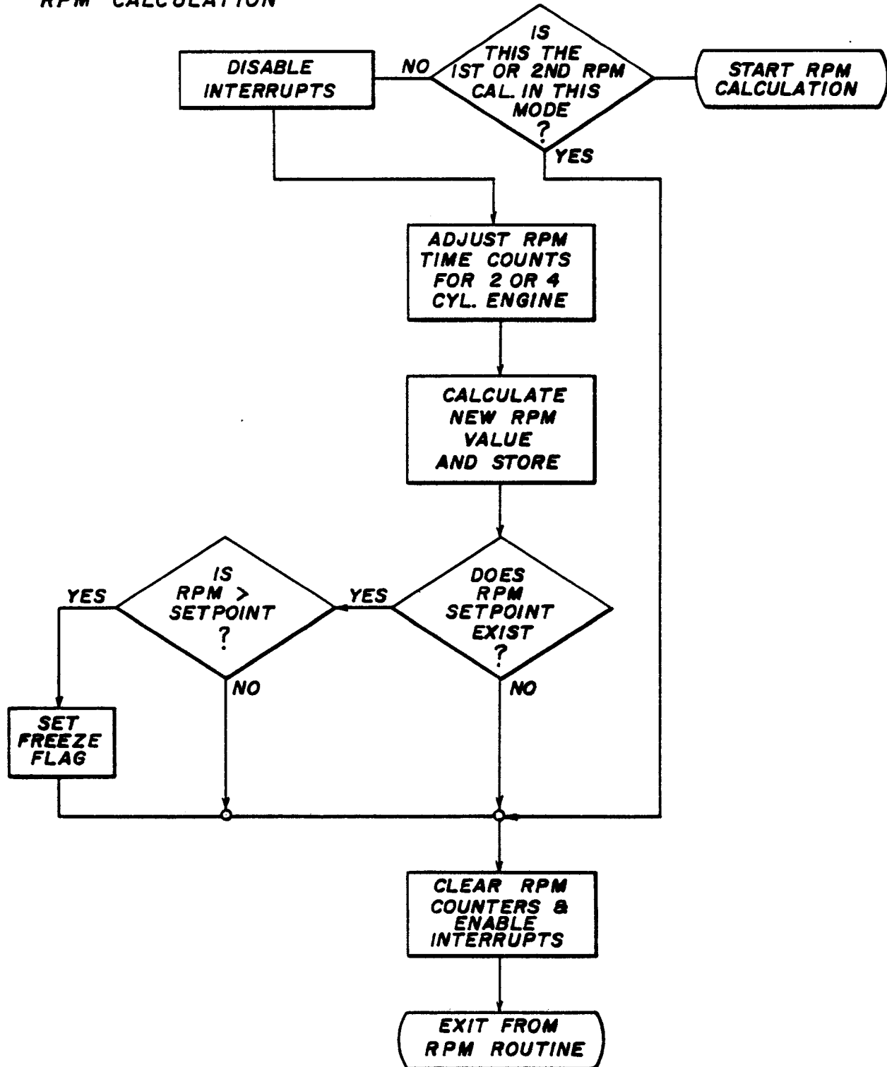
FIG.41C RPM CALCULATION
