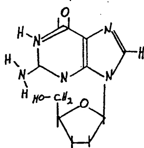
ddG
