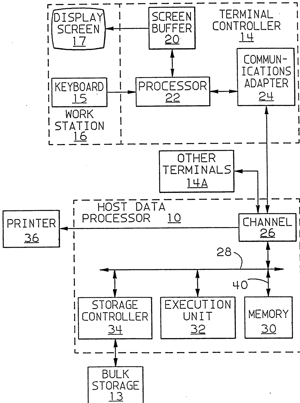
FIG. 6 SYSTEM BLOCK DIAGRAM
