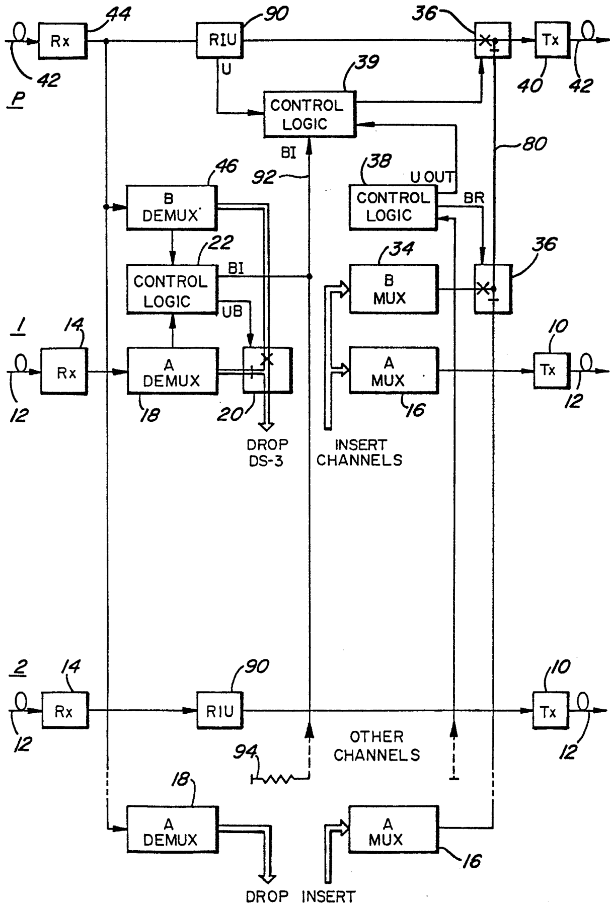
FIG. 6 OPTIONAL EXTRA DS-3 CHANNELS
