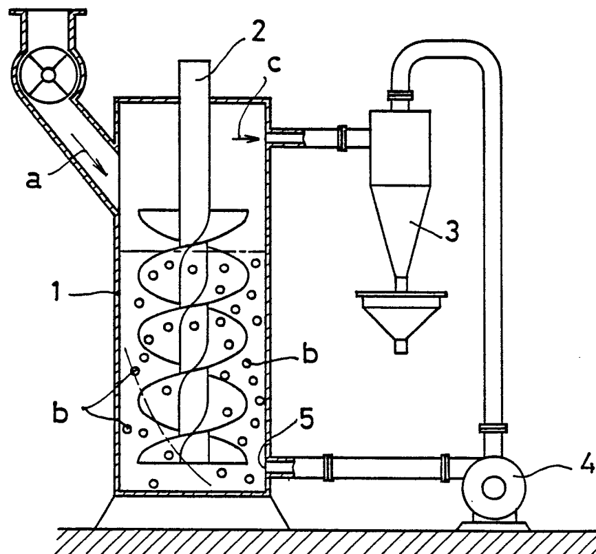
FIG.7 PRIOR ART
