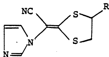
(E isomer)
