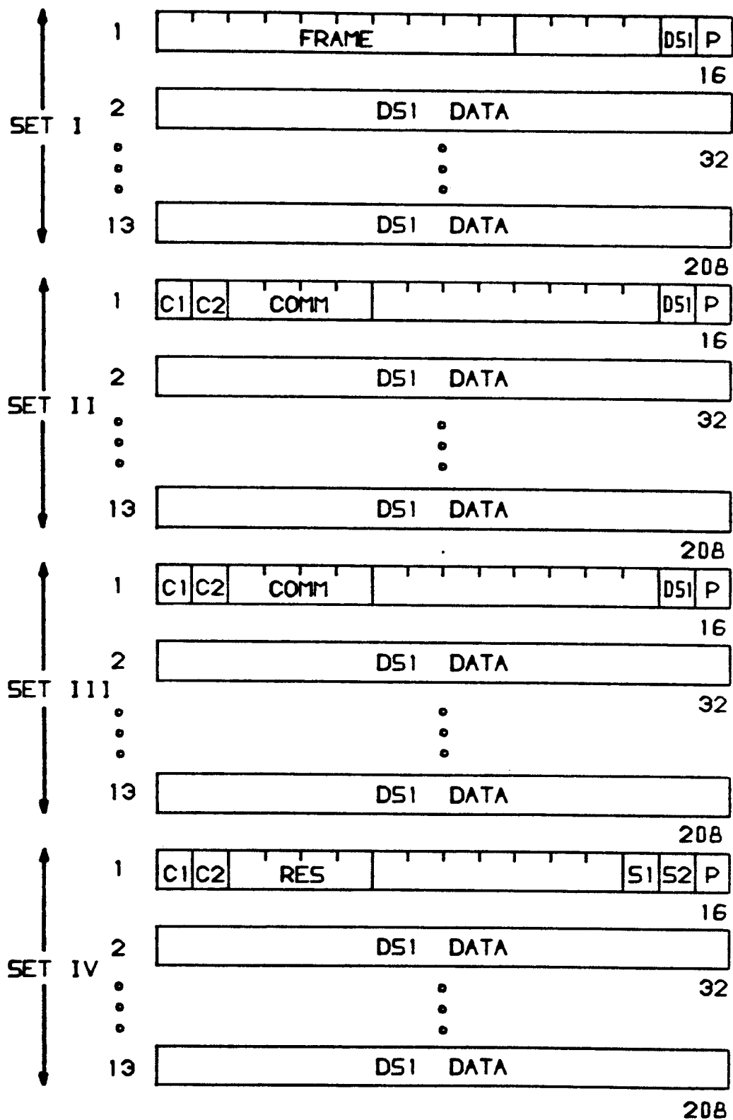
FIG. 4 CHANNEL FRAME FOR DLU-1
