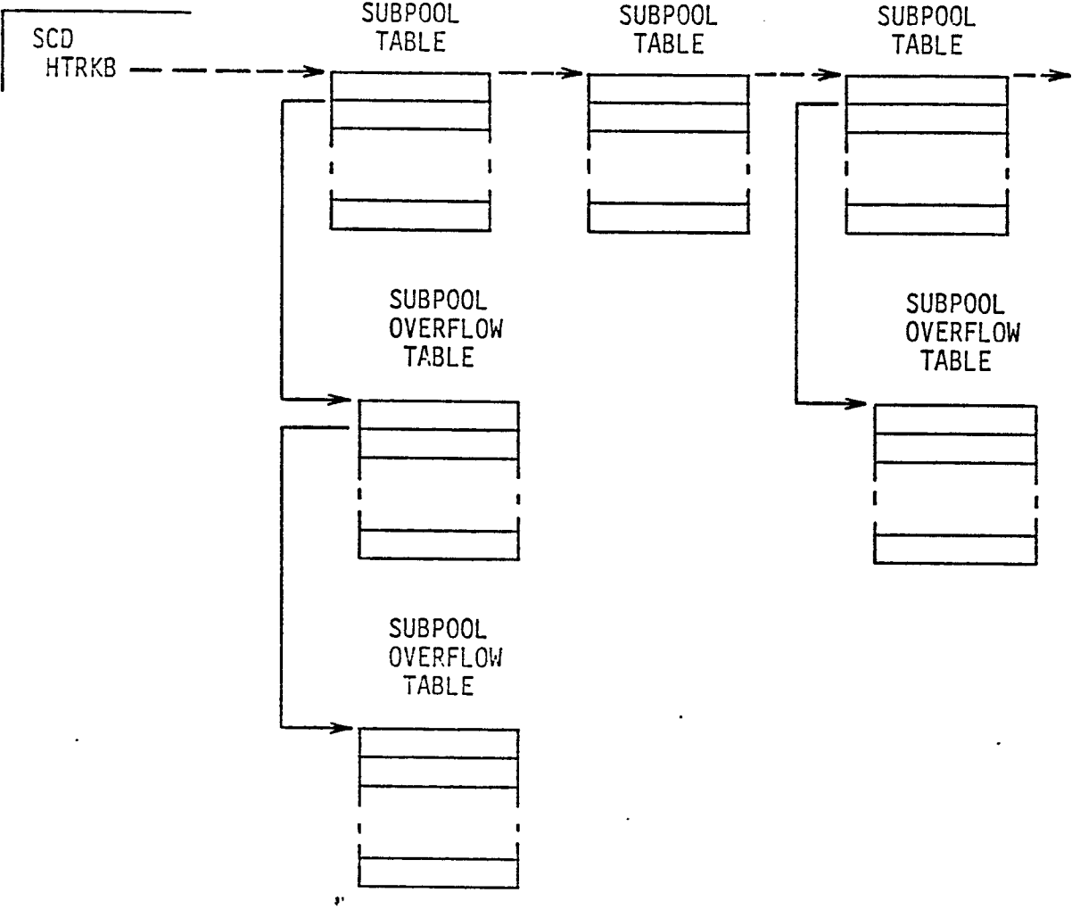
DL/I BUFFER TRACKING POOL STRUCTURE
