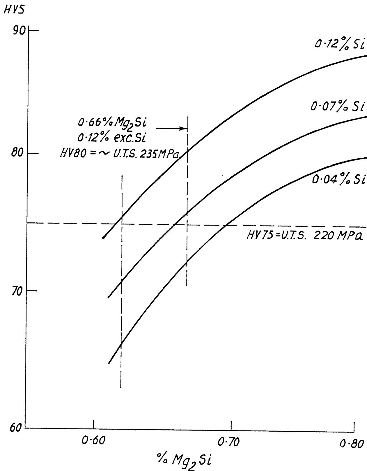
FIG. 2 EFFECT OF Mg_2Si + EXCESS Si ON MAXIMUM HARDNESS OBTAINABLE FROM 6063 ALLOY. SPECIMENS FROM D.C. INGOT. HOMOGENISED, REHEATED, QUENCHED, AGED TO T6
