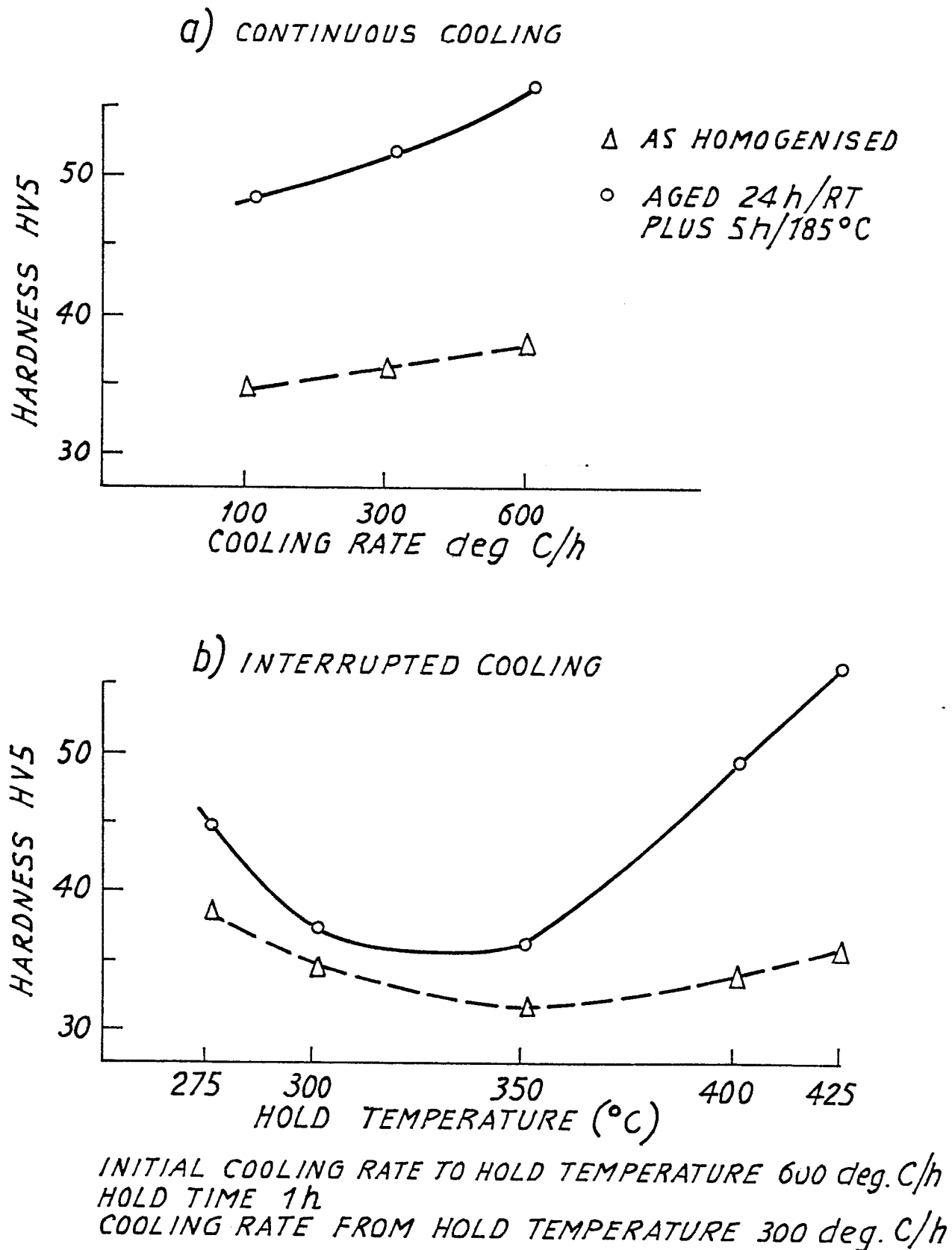
FIG.4 CHARACTERISATION OF AMOUNT OF Mg_2Si PRECIPITATED ON COOLING FROM HOMOGENISATION 2h/585°C BY HARDNESS MEASUREMENT BEFORE AND AFTER AGEING
