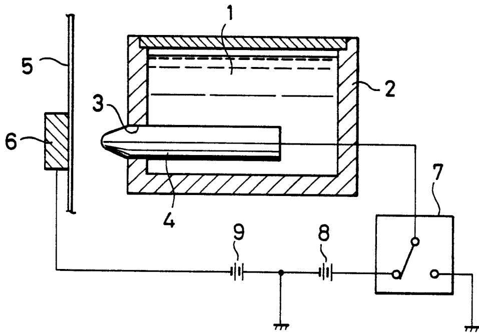
FIG . 7 (PRIOR ART)
