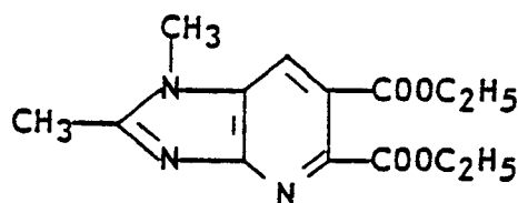
Isomer B
