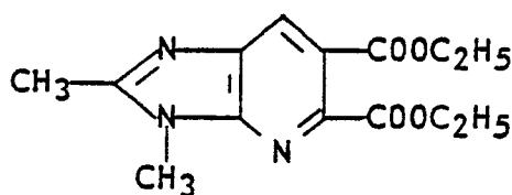
Isomer A
