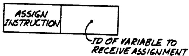
FIG. 17 ASSIGN INSTRUCTION
