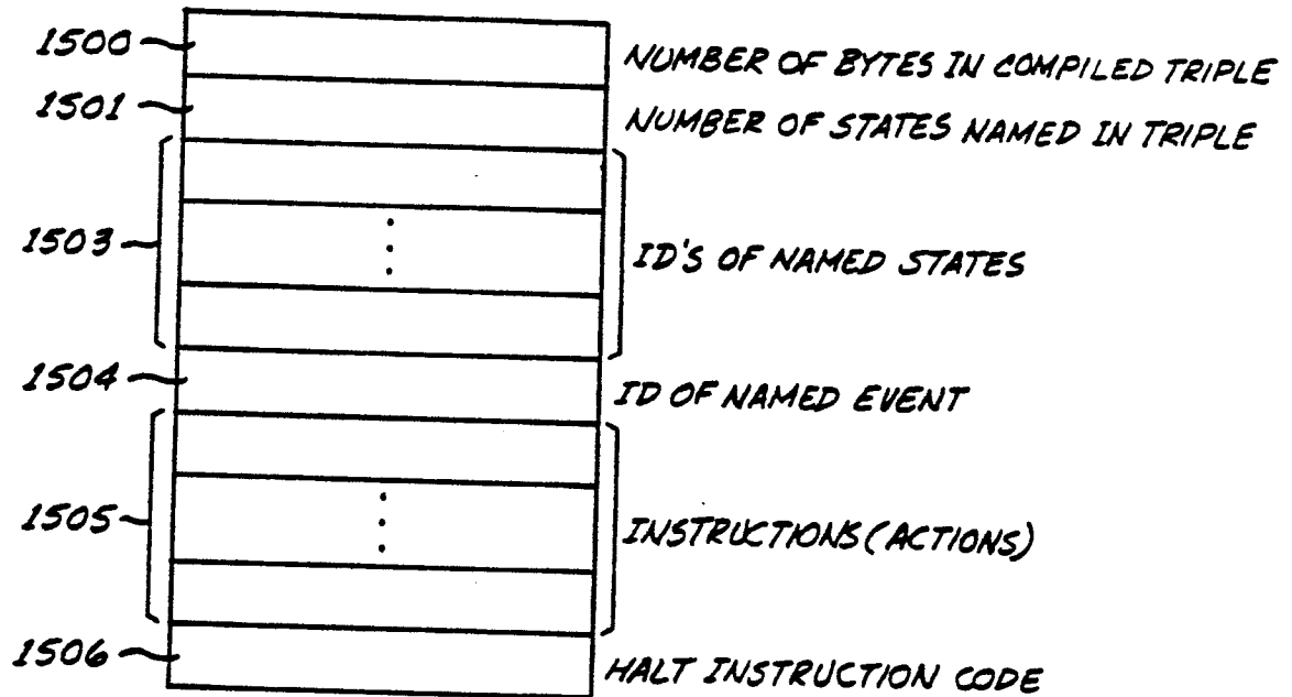
FIG. 15 FORMAT OF COMPILED TRIPLE
