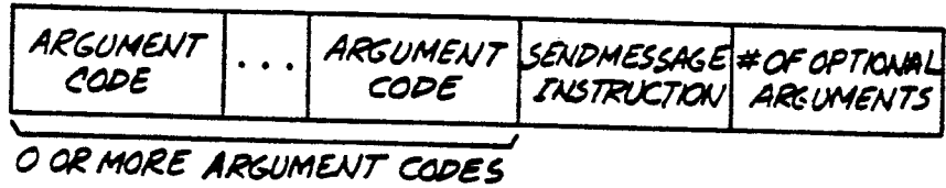
FIG. 18 "SENDMESSAGE" INSTRUCTION
