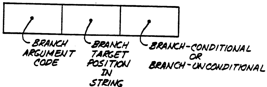
FIG. 21 BRANCH INSTRUCTION
