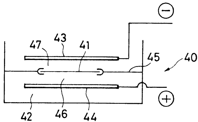
FIG. 4 PRIOR ART
