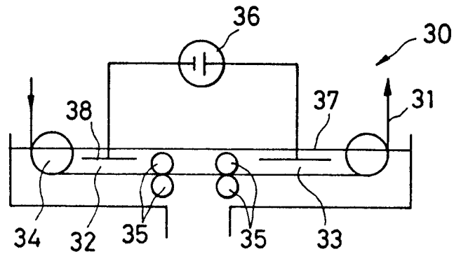
FIG. 3 PRIOR ART
