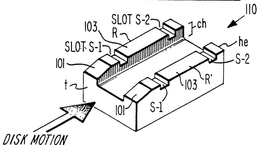
FIG. 7. MODIFIED 3680 SLIDER FOR BURNISHING.
