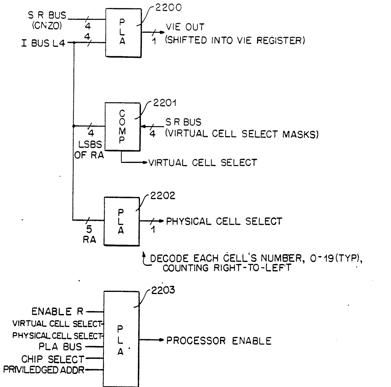
PROCESSOR ENABLE PLA STATE TABLE
