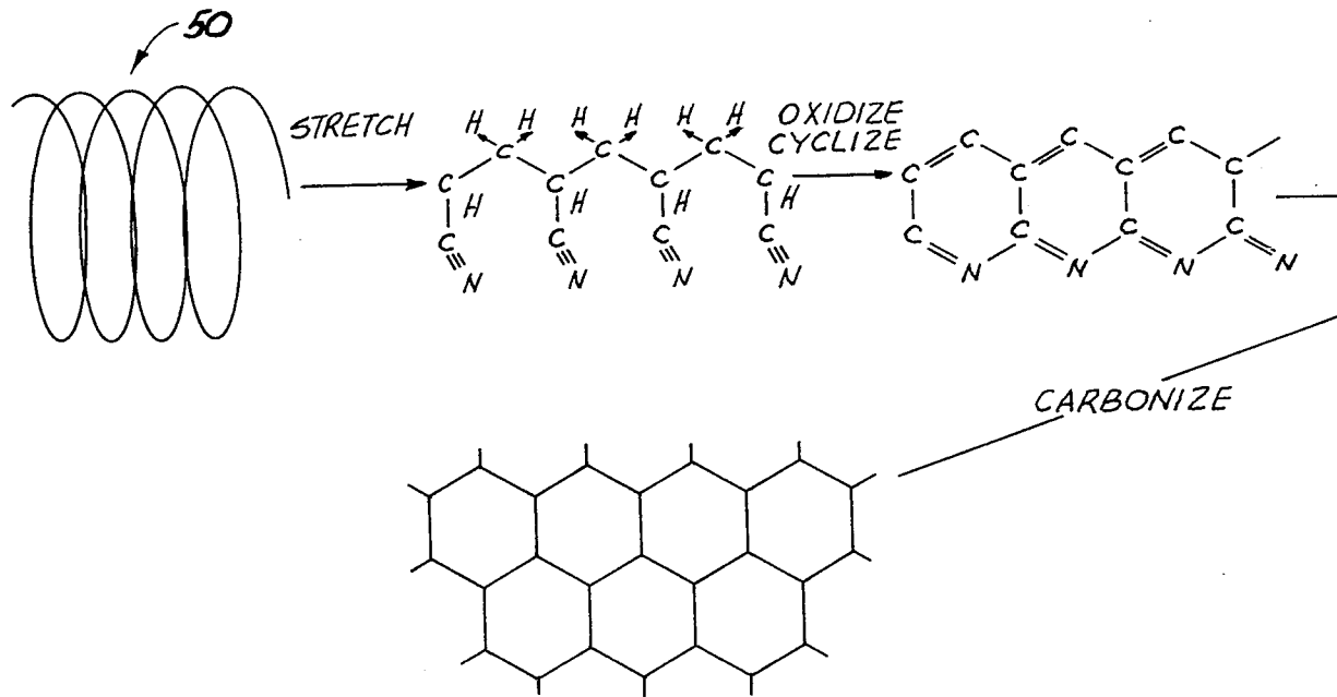
Fig. 1 (PRIOR ART)
