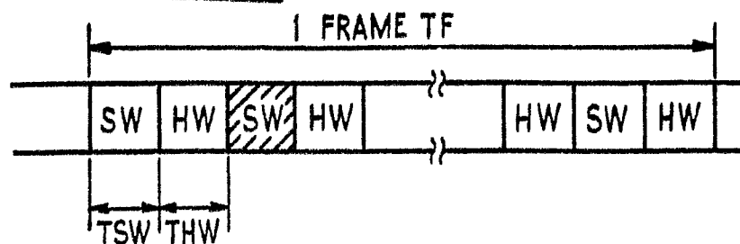
FIG. 1 (PRIOR ART)
