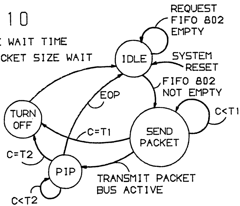
OUTPUT CONTROLLER 803
