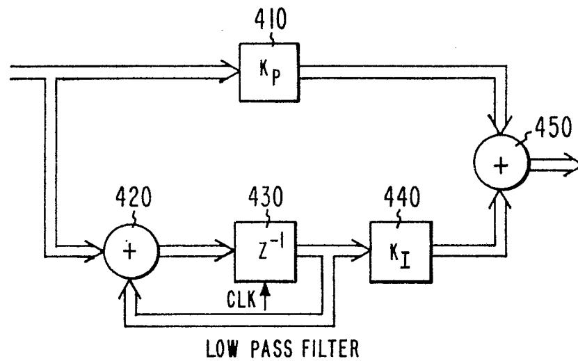
Fig. 4 PRIOR ART
