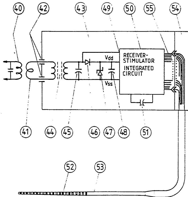
Implantable Receiver/Stimulator FIG. 5
