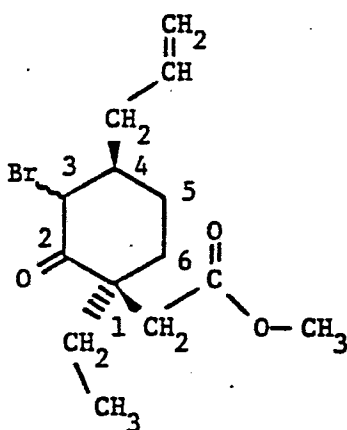
(IVa-( \pm ) cis )
