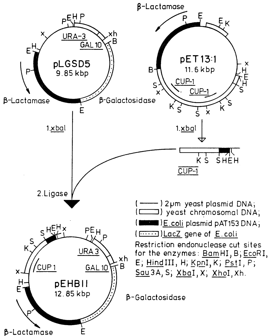
Fig.1. Construction of plasmid pEHBII
