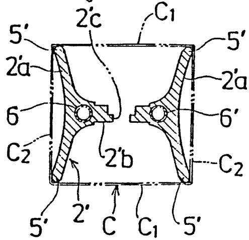
Fig. 9 Prior Art
