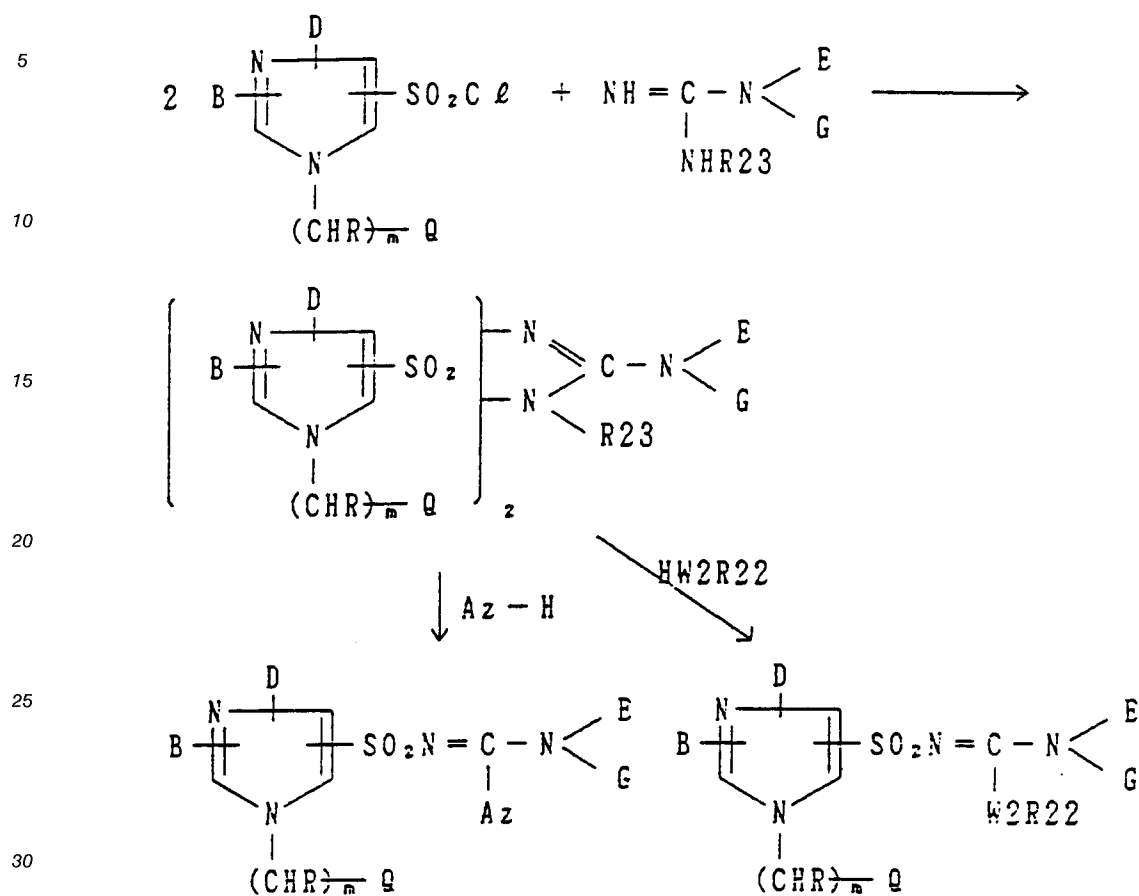
Reaction scheme 5
