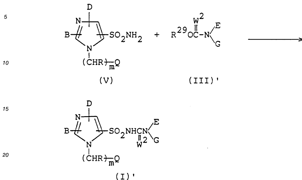
Reaction scheme 3
