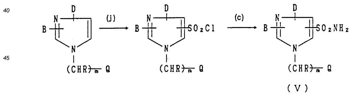
Reaction scheme 10
