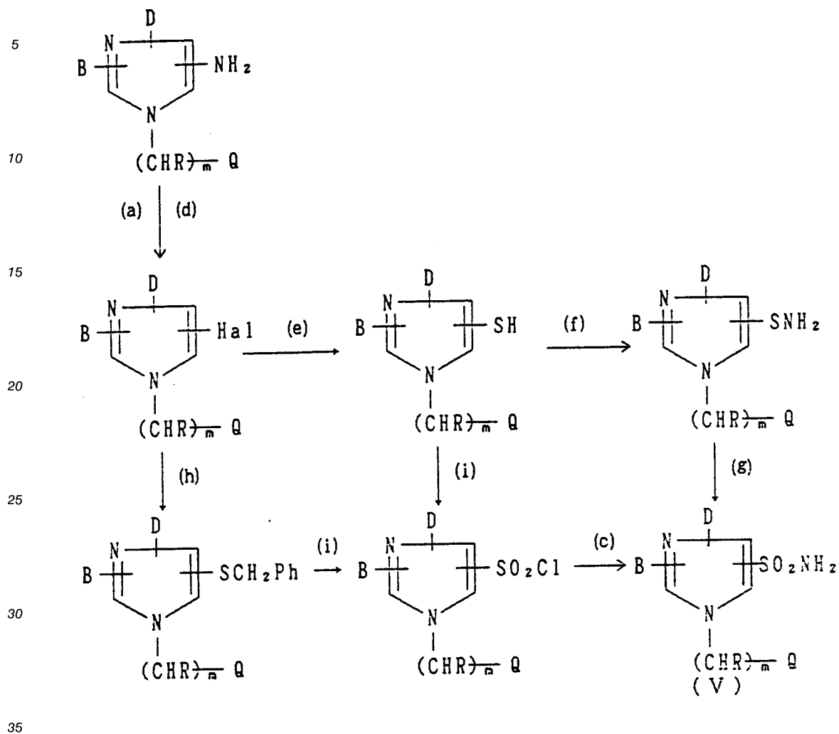
Reaction scheme 10
