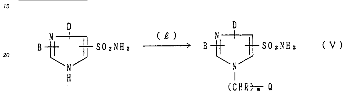
Reaction scheme 12
