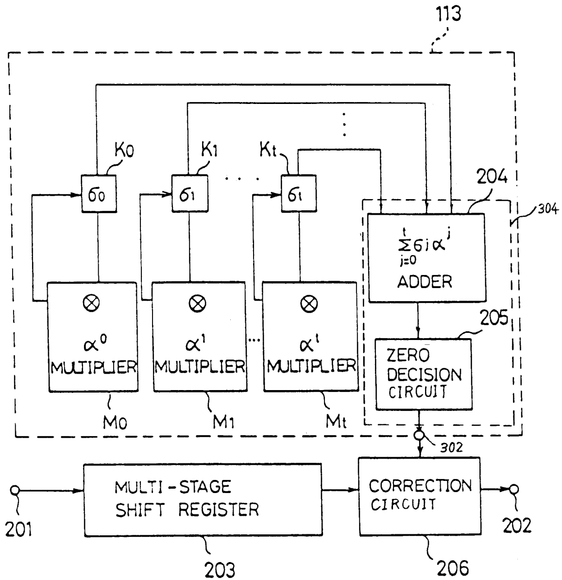
FIG. 15 PRIOR ART
