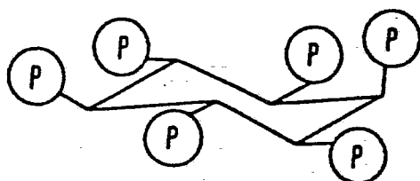
1.2.3.4.5.6-hexakis-(dihydrogen-phosphate)-myo-inositol alternatively myo-inositol hexakis (phosphate) or IP_6
