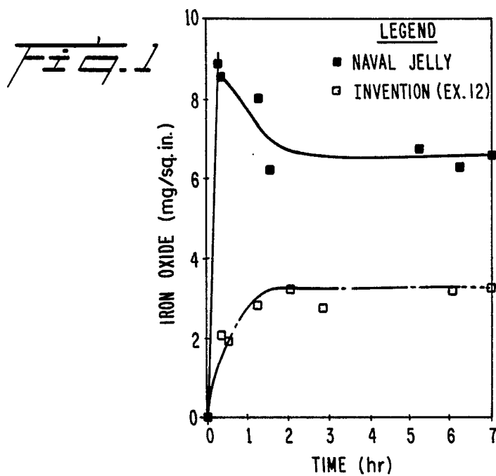
RUST REMOVAL vs. TIME FOR PRODUCT COATINGS
