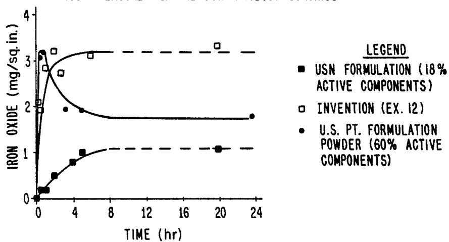
RUST REMOVAL vs. TIME FOR PRODUCT COATINGS
