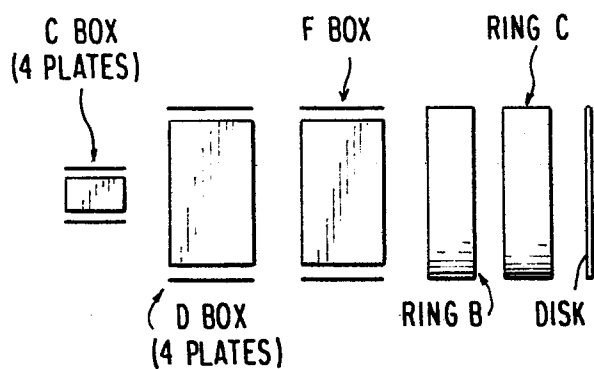
FIG. 5A (PRIOR ART) 12 PLATE SYSTEM
