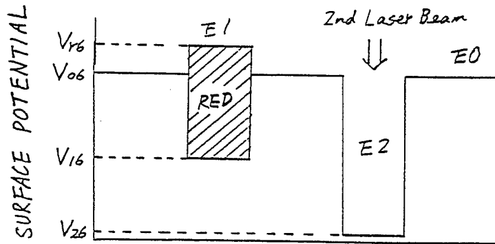
Fig. 2E (AFTER 2nd EXPOSURE)
