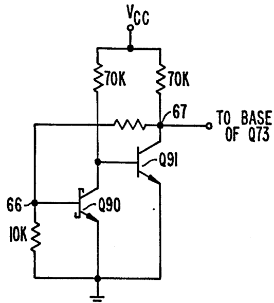
FIG. 6B. HYSTERESIS AMPLIFIER
