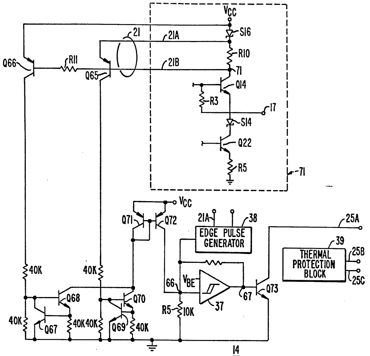
FIG. 6A. CURRENT LIMITER SECTION
