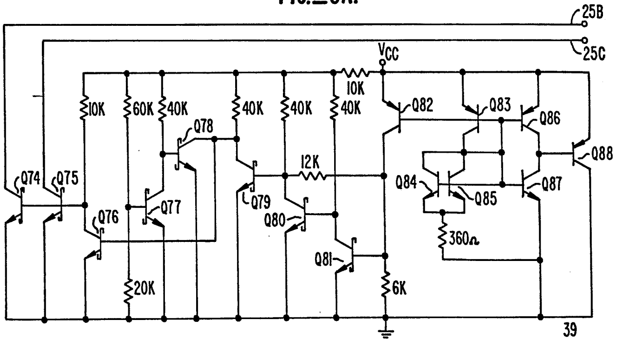
THERMAL SHUTDOWN CIRCUIT
