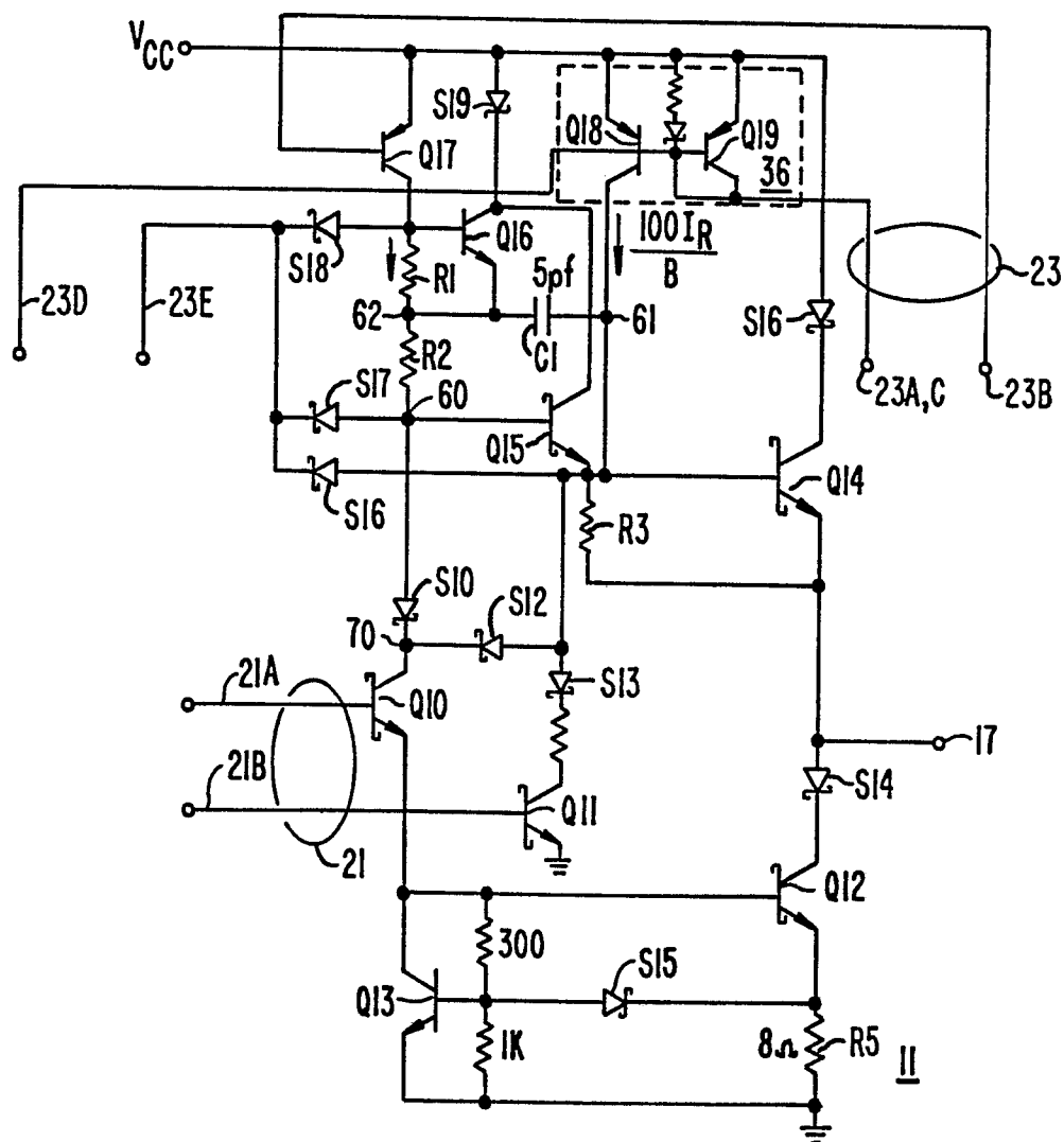
DRIVER SECTION FIG. 3A.
