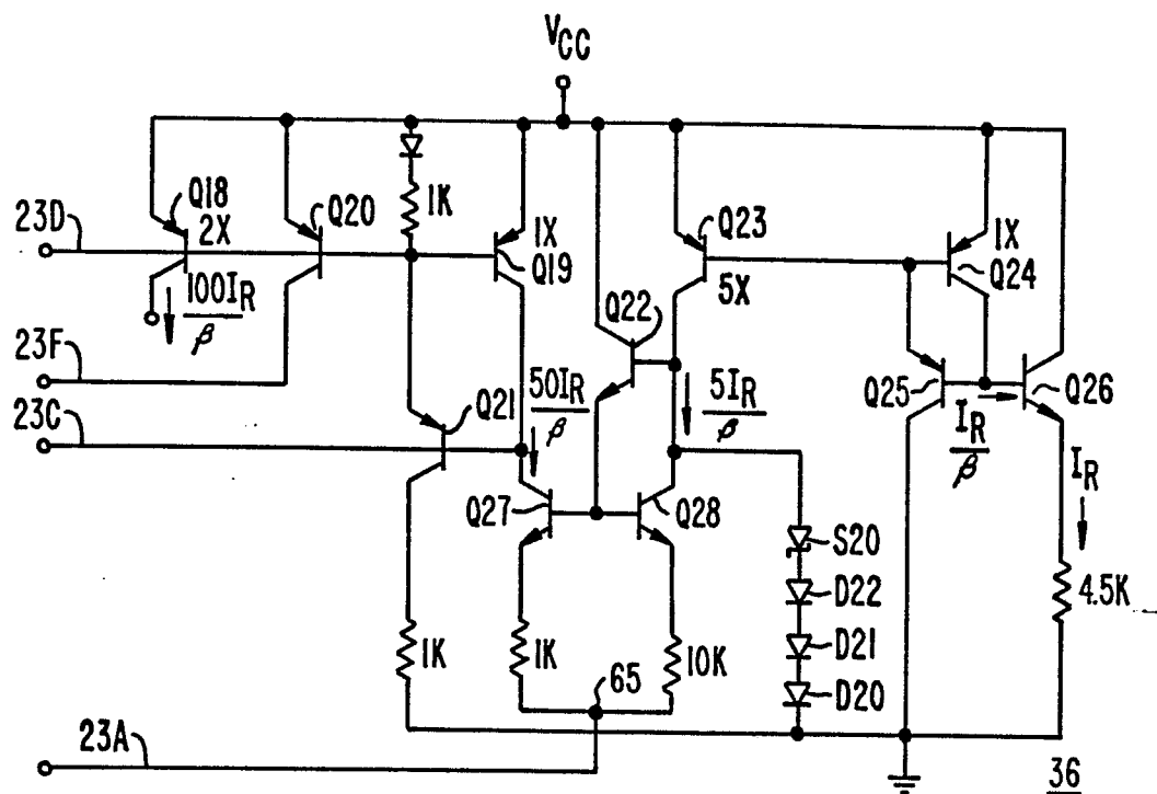
REFERENCE CURRENT SOURCE BLOCK
