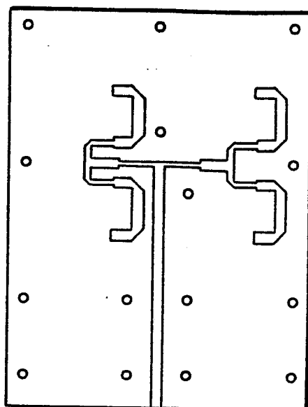
FIG. 15b POWER DIVIDING NETWORK
