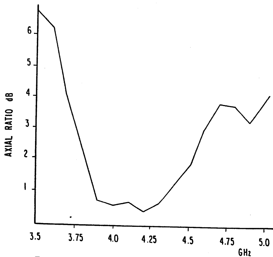
FIG. 7 - AXIAL RATIO OF 4-ELEMENT ARRAY
