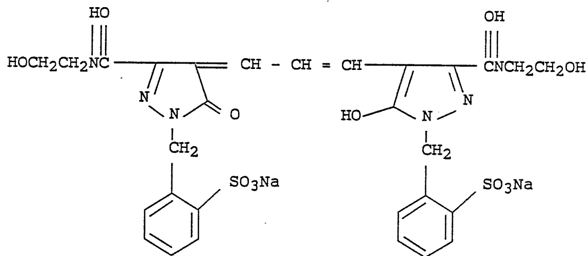
Compound E x - 3b
