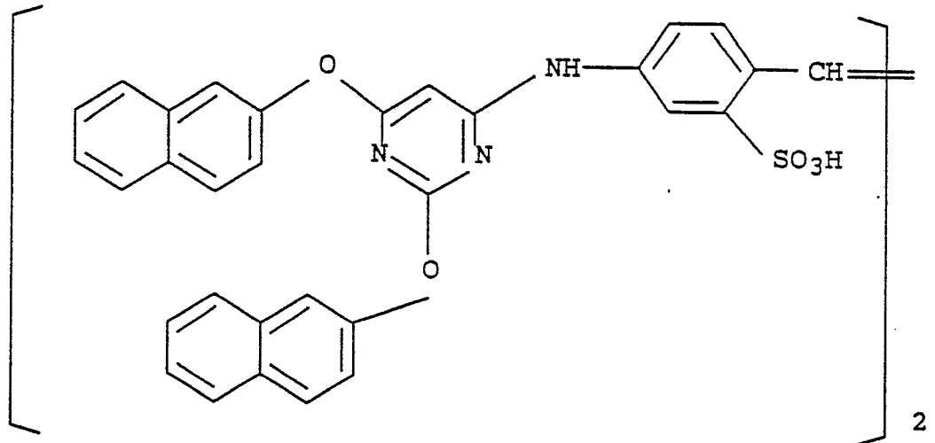
Compound Ex - 3c
