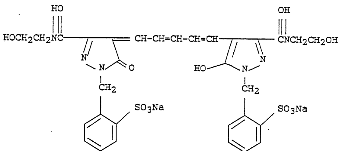
Compound E x - 3a
