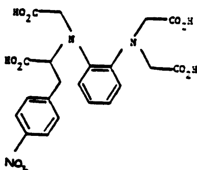
N-(carboxymethyl)-N-(2-(bis(carboxymethyl)amino) phenyl)-(4-nitrophenyl)alanine
