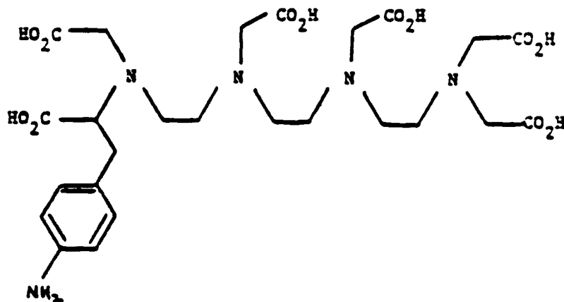
N-(carboxymethyl)-N-(2-aminoethyl)-N'-(carboxymethyl)-N'-(2'-aminoethyl)-N''-(carboxymethyl)-N''-(2''-(bis(carboxymethyl)amino)ethyl)-(4-aminophenyl)alanine
