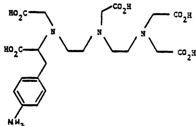
N-(carboxymethyl)-N-(2-aminoethyl)-N'-(carboxymethyl)-N'-(2'-(bis(carboxymethyl)amino)ethyl)-(4-amino-phenyl)alanine
