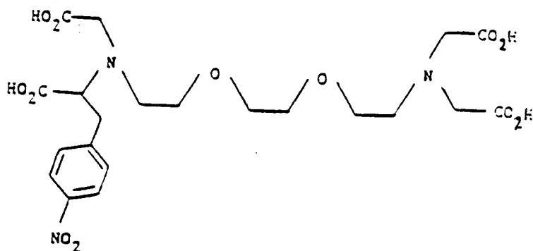
N-(1-carboxy-2-(p-nitrophenyl)-ethyl)-1,8-diamino-3,6-dioxaoctane-N,N',N'-triacetic acid.
