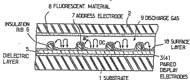
FIG. 1 CROSS-SECTIONAL VIEW OF SURFACE-DISCHARGE TYPE GAS-DISCHARGE PANEL
