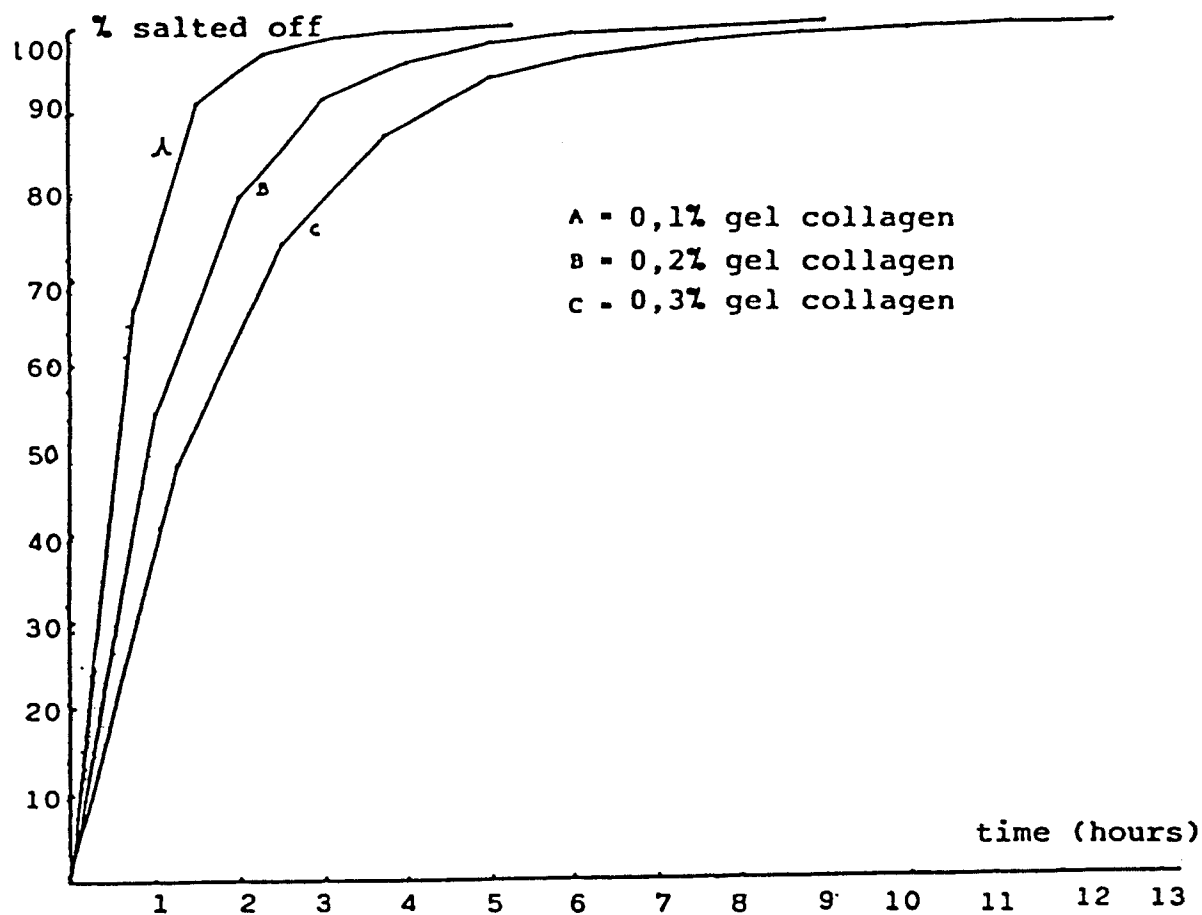
FIG.3 - Proceeding of salting off in time versus collagen gel having 0.1-0.2 and 0.3% concentrations.
