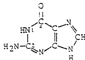
Guanine (2-amino-6-oxypurine)
