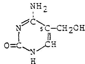
5-Hydroxymethylcytosine
