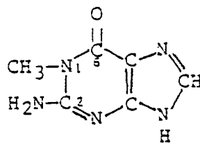
1-Methylguanine
