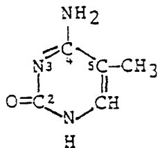
5-Methylcytosine
