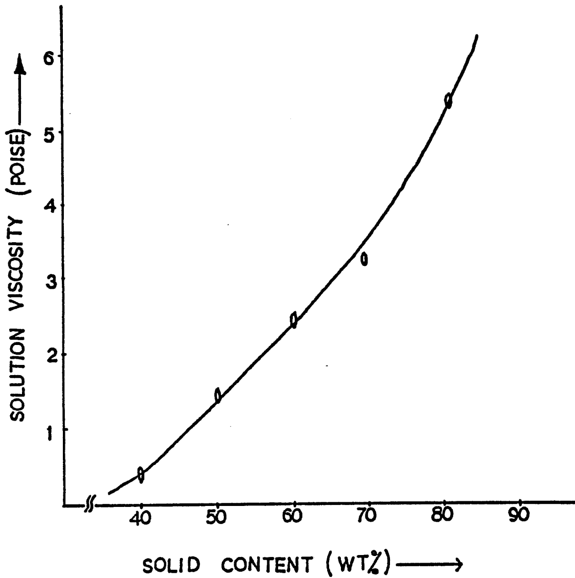
FIG. 4 Solution Viscosity vs. Solid Content of G4
