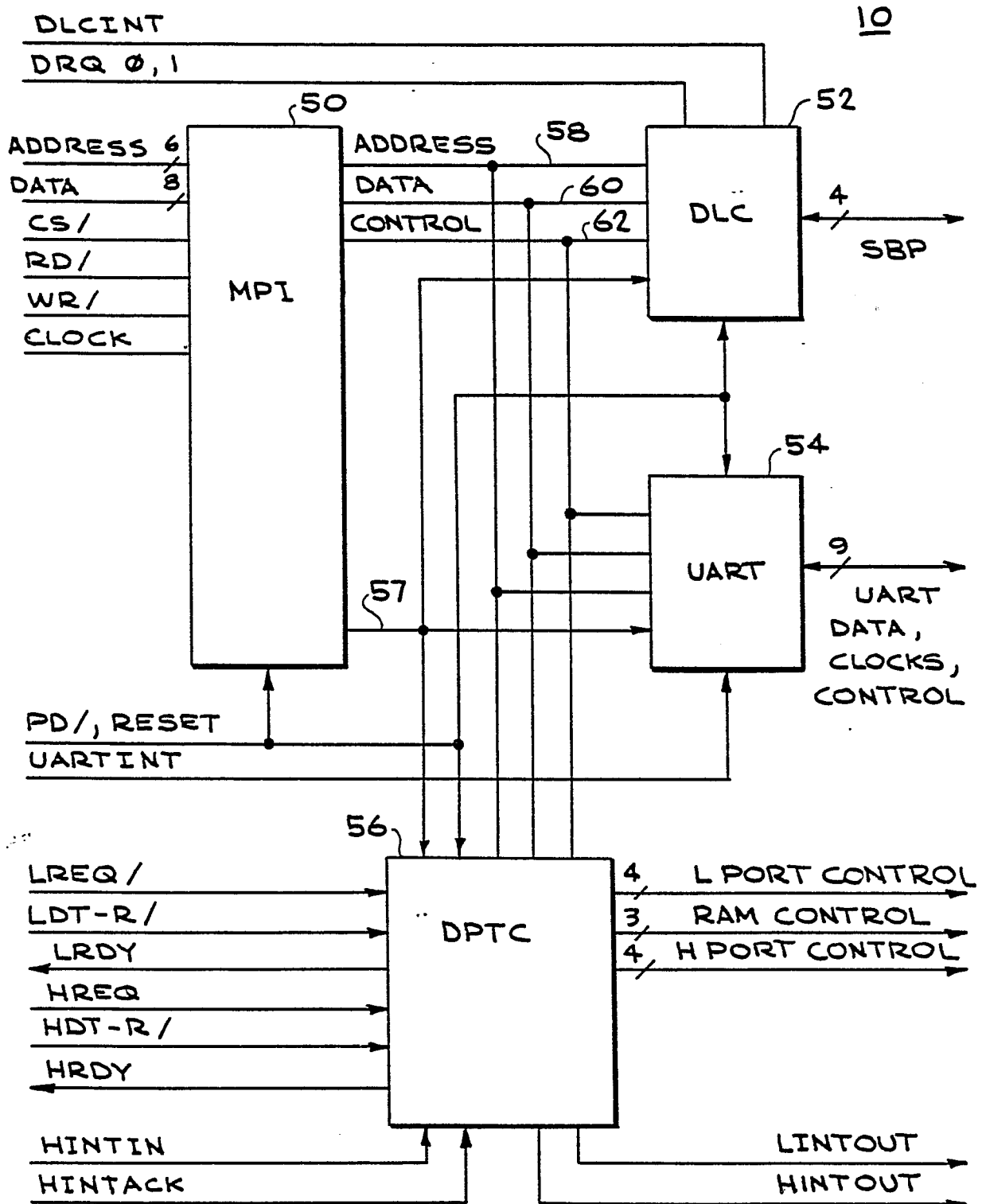
IDPC BLOCK DIAGRAM
