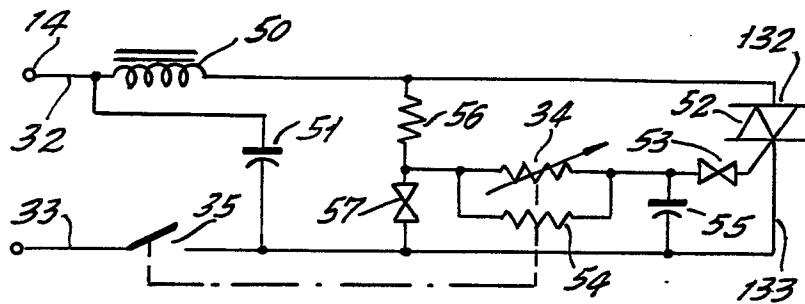
FIG. 7. PRIOR ART
