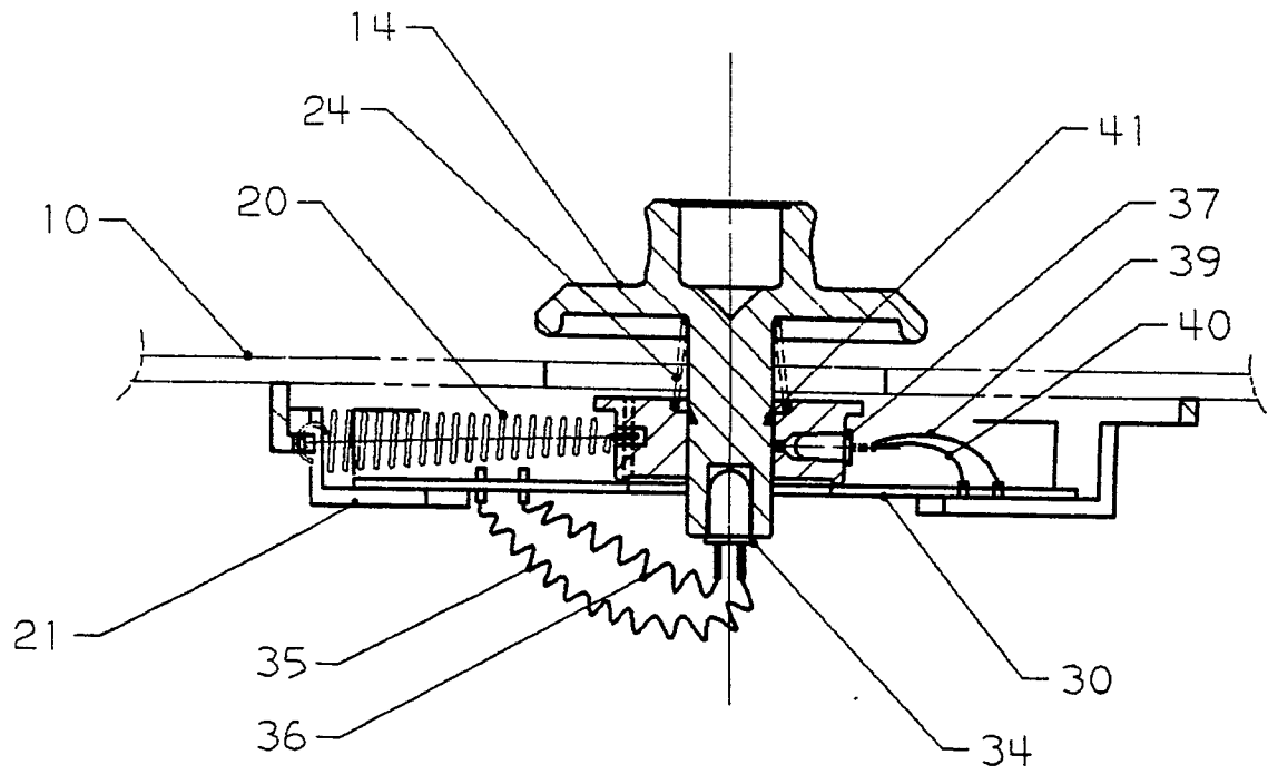
SECTION B-B - FIG 4
