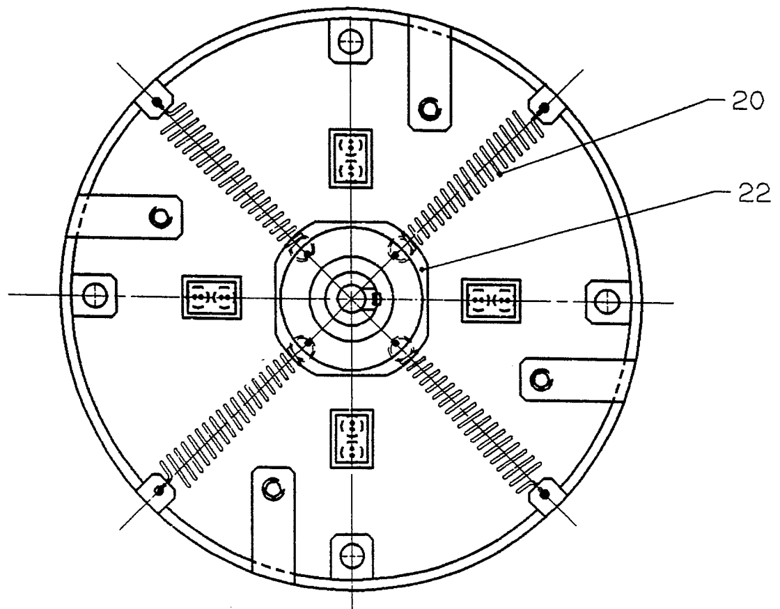
SECTION C-C - FIG 5
