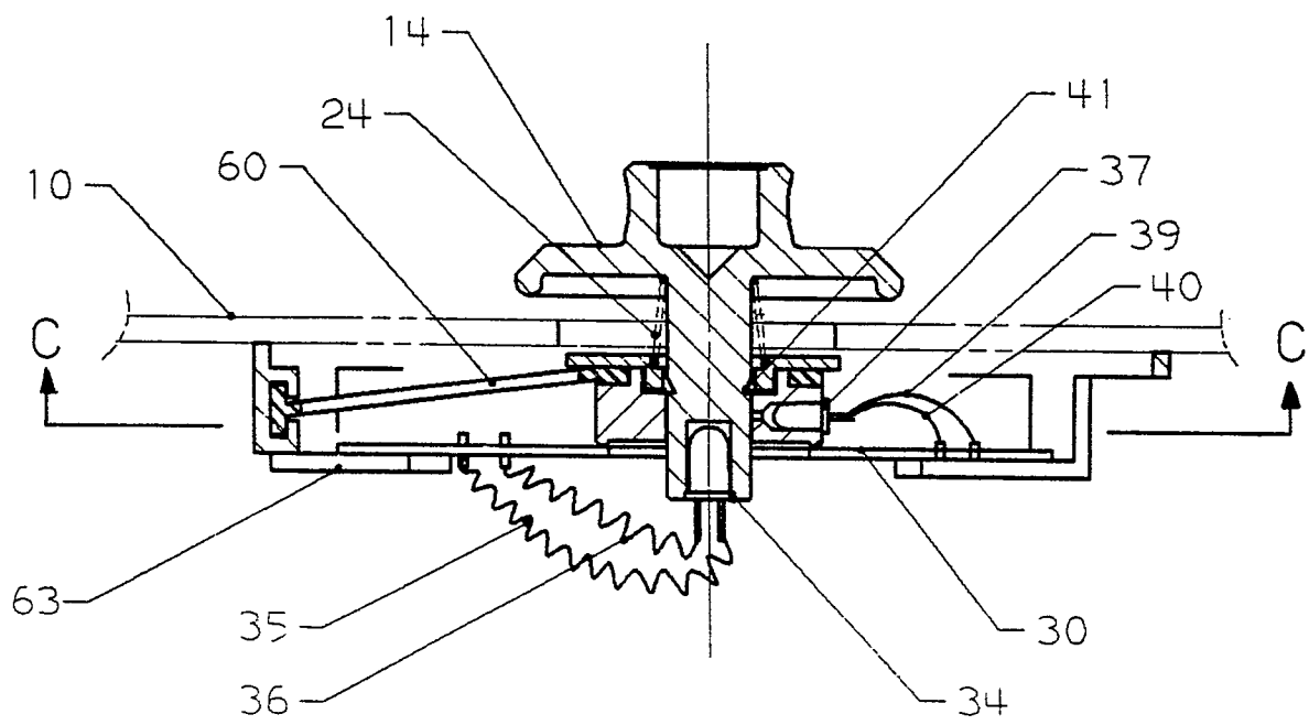
SECTION B-B - FIG 8
