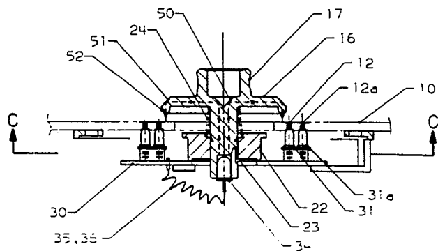
SECTION A-A - FIG 3
