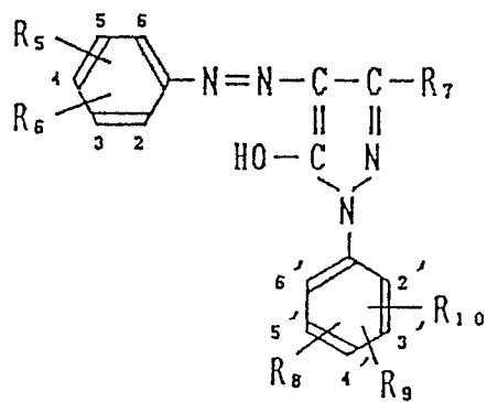
Formula [VI-b]
