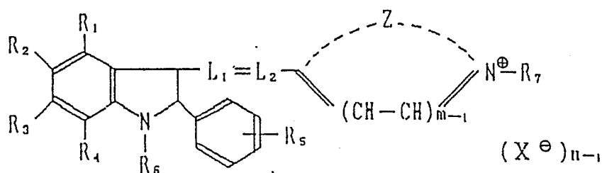
Formula [IV]
