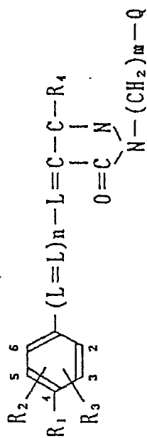
Formula [VI-a]
