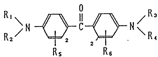
Formula [VI-d]
