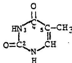
5-Hydroxymethylcytosine
