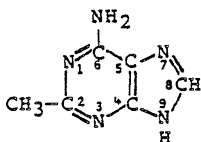
2-Methyladenine
