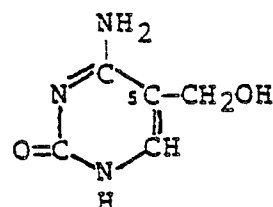
5-Hydroxymethylcytosine
