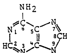
Adenine (6-aminopurine)
