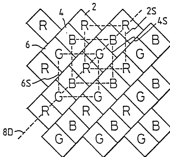
DIAGRAM OF FIRST EMBODIMENT OF COLOR PICTURE ELEMENT ARRAY
