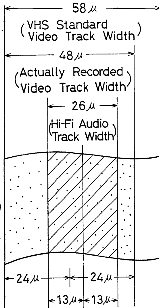
Fig. 5(a) (Self-recording & Self-reproduction)
