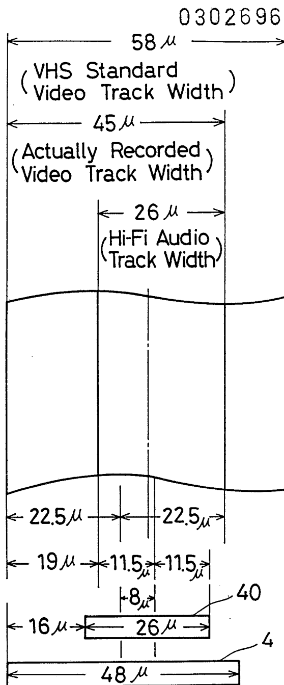
Fig. 6(a) (Borrowed-recording & Borrowed-reproduction)
